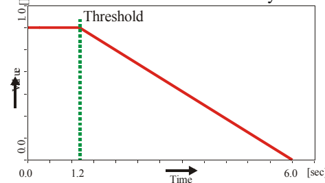
Figure 4: Relation of the time interval \delta t between two strokes and the connectivity value.
